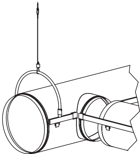
Middle aligned branch with extended strap length
