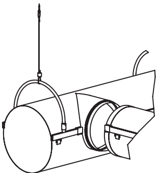
Branches Top/center/bottom aligned
