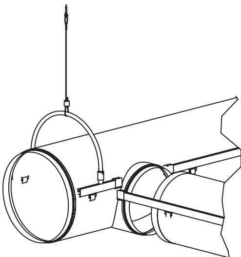
Bottom aligned branch with extended strap length
