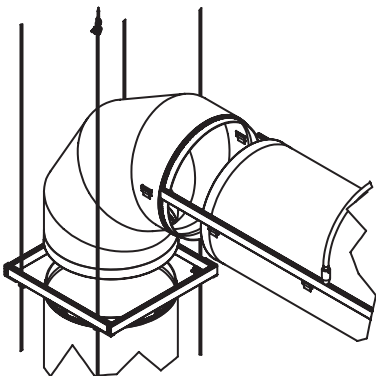
Vertical duct suspension methods
