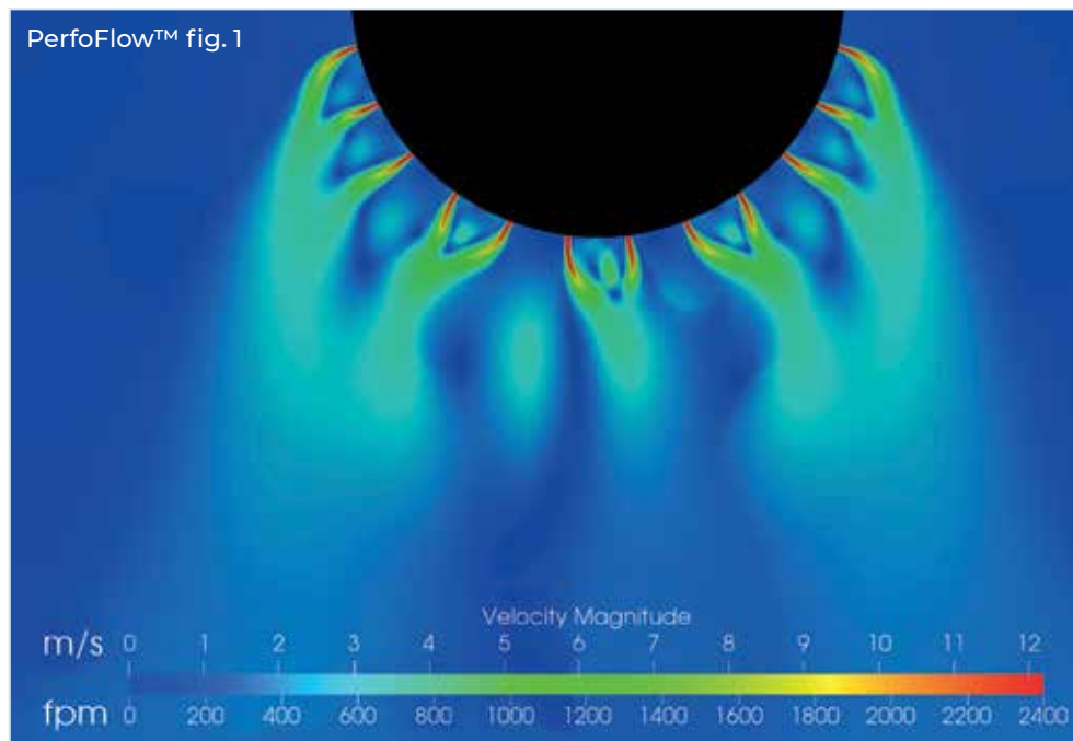
Air discharge through PerfoFlow™ perforation at 120 Pa [0.48 inwg].
