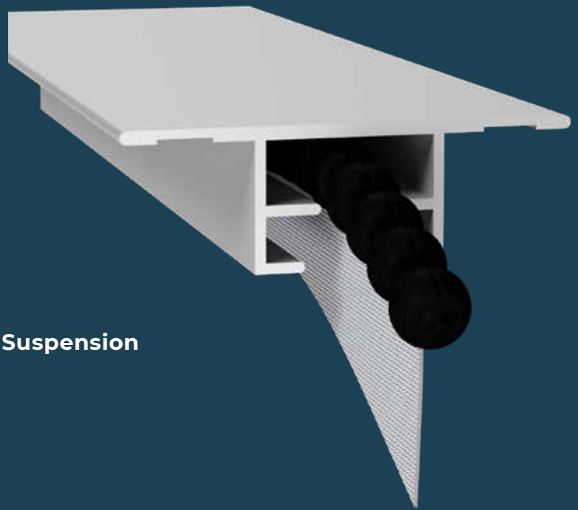
H-rail Suspension
