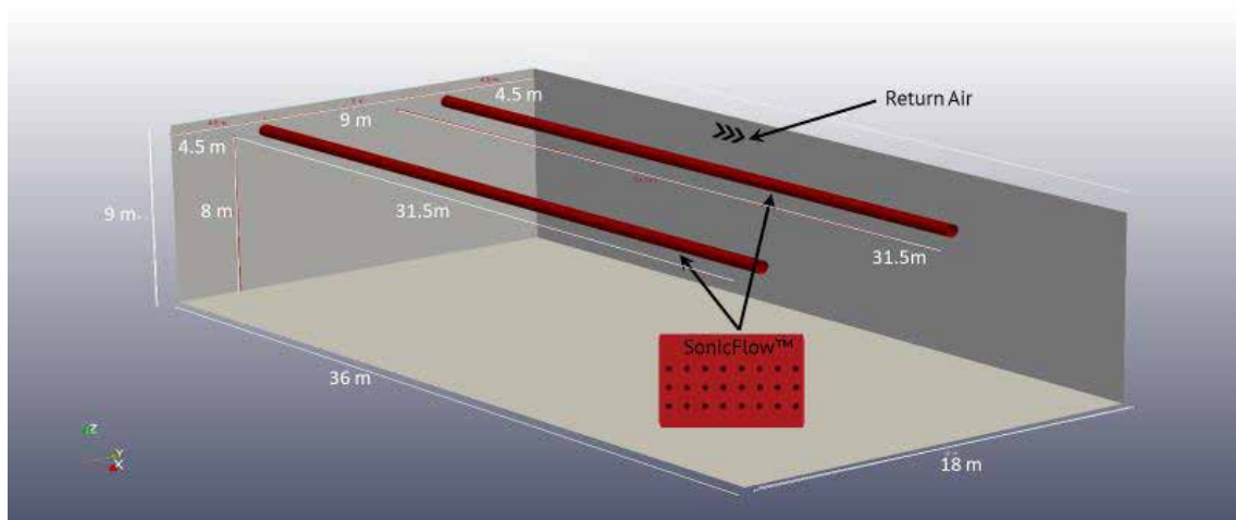
Figure 2. Simplified room geometry used for CFD simulations
