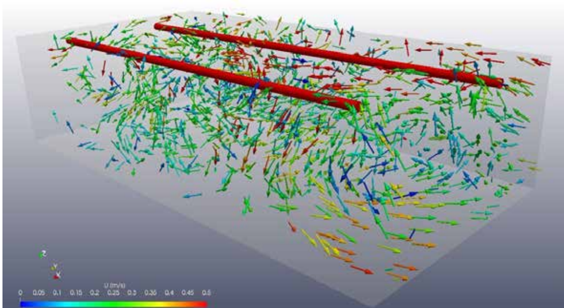
Figure 7. Circulation of air in the building
