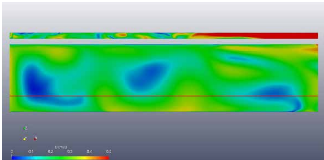
Figure 5. Longitudinal section view. Air velocities (scale 0-0.5 m/s).
